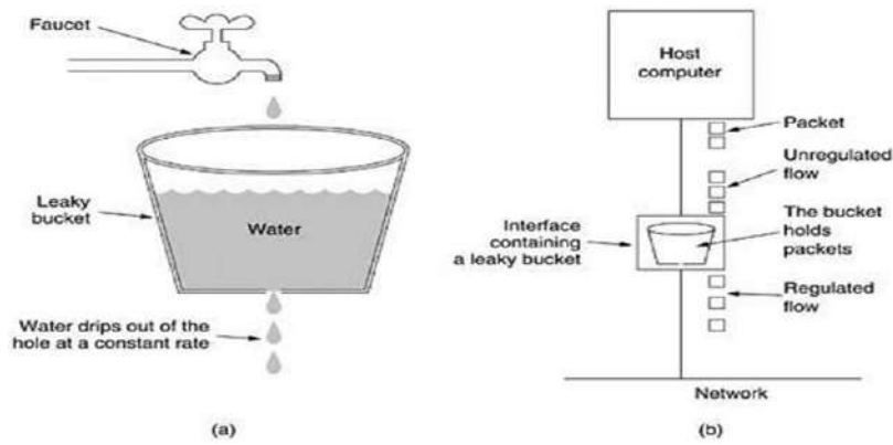
Figure 12 Leaky Bucket Algorithm
