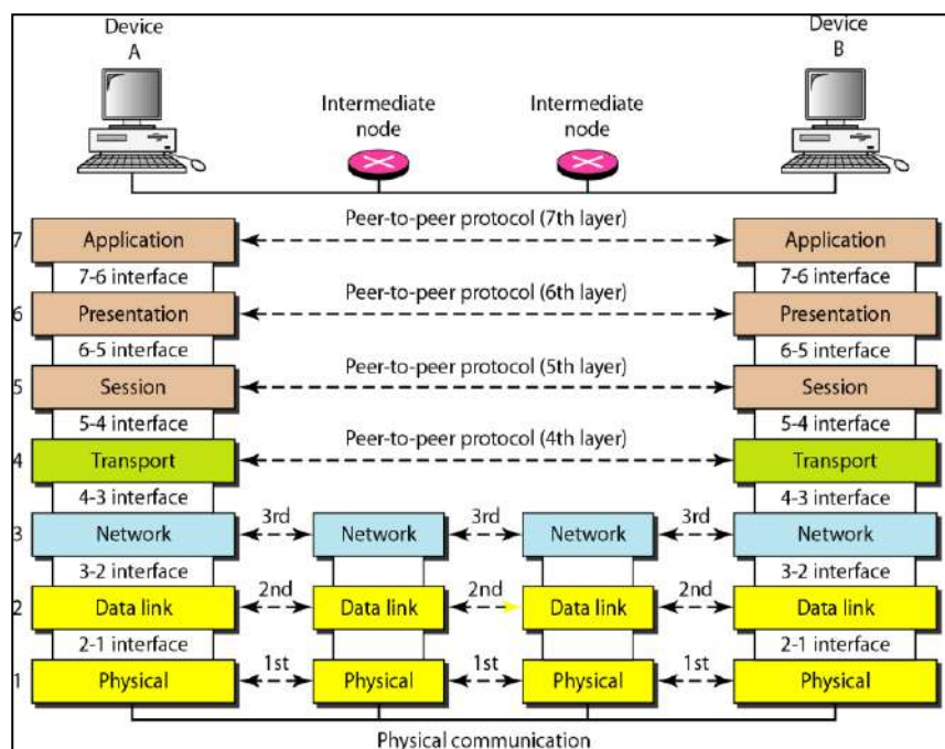
Figure 3 The interaction between layers in OSI Model
