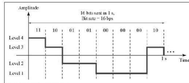
Figure 4 Digital Signal with four levels
