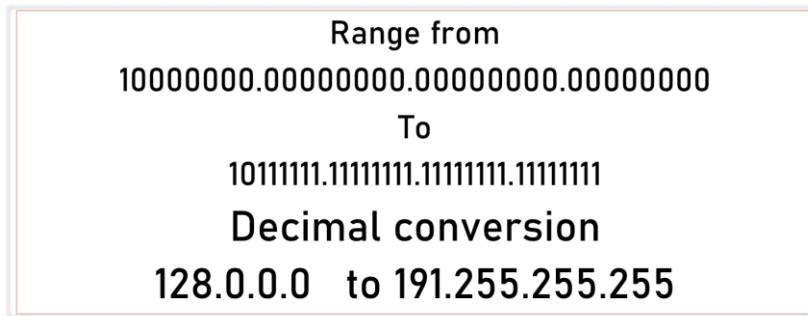
Figure 18 Conversion to Decimal Notation
