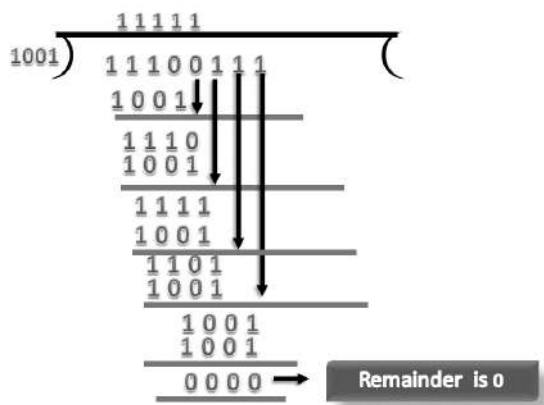
Figure 17 CRC Checker
