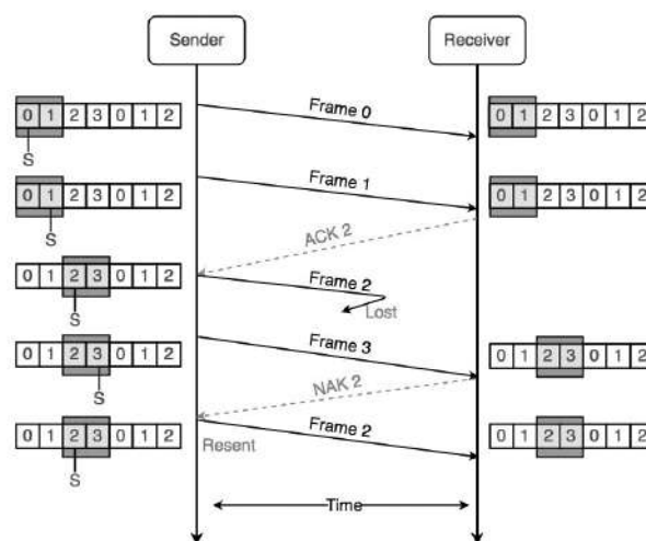
Figure 30 Selective Repeat Protocol
