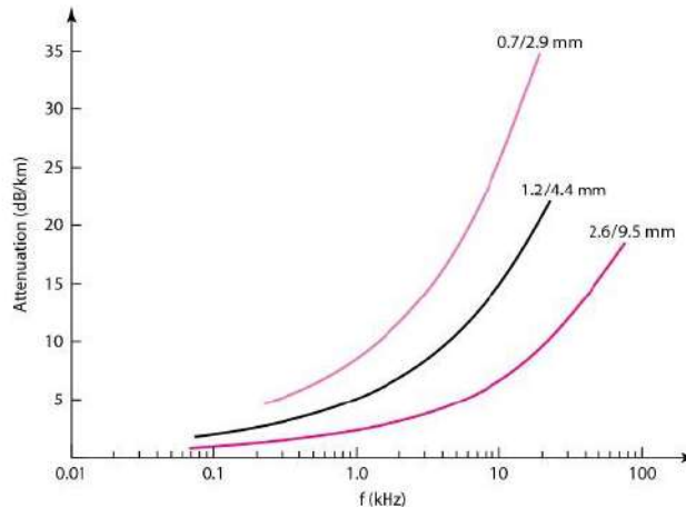
Figure 7 Performance of coaxial cable
