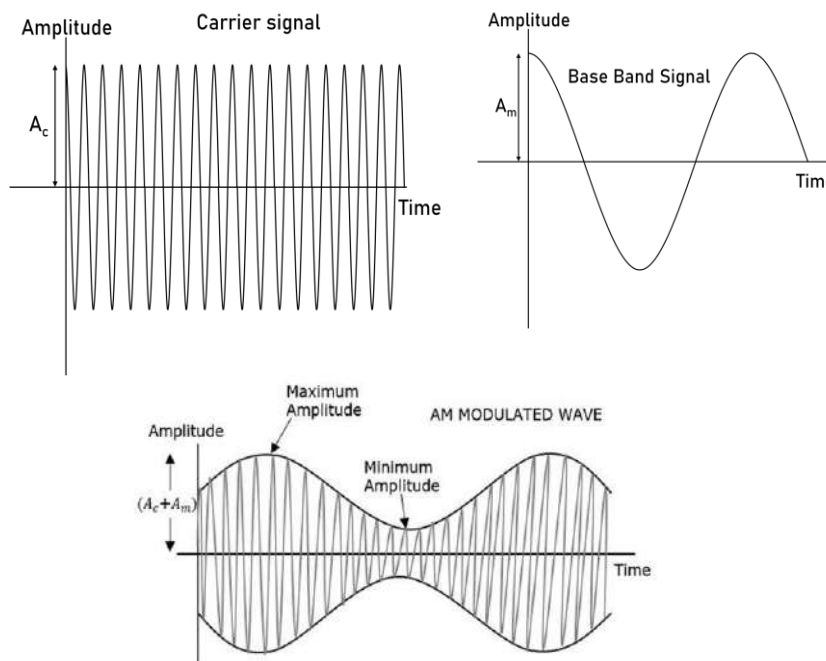
Figure 16: Amplitude Modulation
